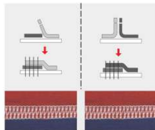
单切车缝 Single cut sewing 双切车缝 Double cut sewing
