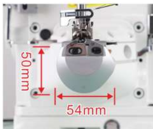
一体式针板 Integrated needle plate
