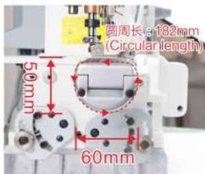
细筒型设计 Slim barrel design
